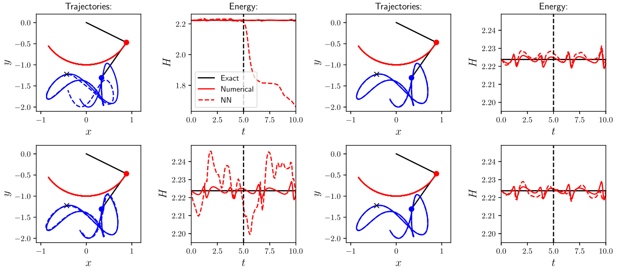
Fig. 11. Comparison of the predictions of one MLP, SympNet, H  nonNet and GHNN (from top left, top right, to bottom right) for one exemplary test trajectory of the double pendulum. The solid lines are the data and the dashed lines the predictions. The black dashed line in the energy plots and the black cross in the trajectory plots indicate where the training data ends.
